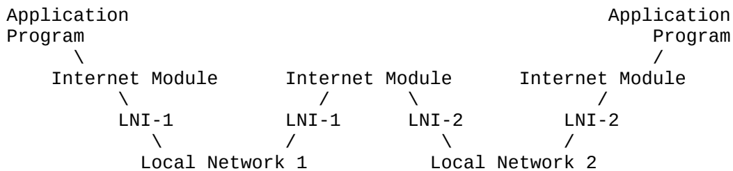
Transmission Path
