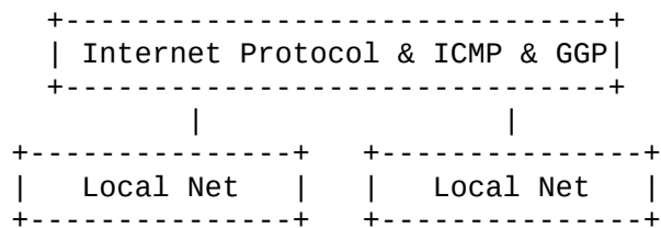
Gateway Protocols
